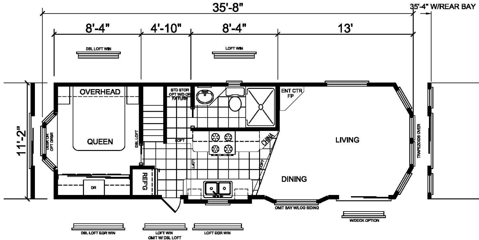
APH-422 - SPORTSMAN'S LODGE 399 SQ FT
